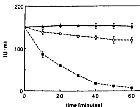
Fig. 2. Inactivation of mitochondrial creatine kinase from chicken heart (Mi b -CK) by CIRATP. Mi b -CK was incubated at 25°C and pH 7.5 for the indicated periods of time. (▲) In the absence of CIRATP; (■) in the presence of 0.25 mM CIRATP; (○) in the presence of 0.25 mM CIRATP + 4 mM ADP. CK activity was measured by the pH-stat method. All data points are given as mean ± SD of 3 measurements.
