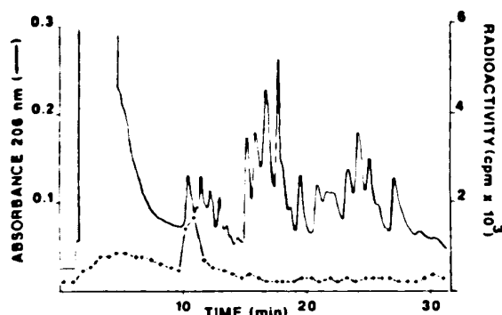
Fig. 3. Reversed phase chromatography profile of the pepsin digest of Mi_b -CK labelled with [ ^{14}C ]CIRATP. The labelling, pepsin digestion, and separation of the peptides obtained were performed as described in section 2. (—) Absorbance at 206 nm; (---) radioactivity.
